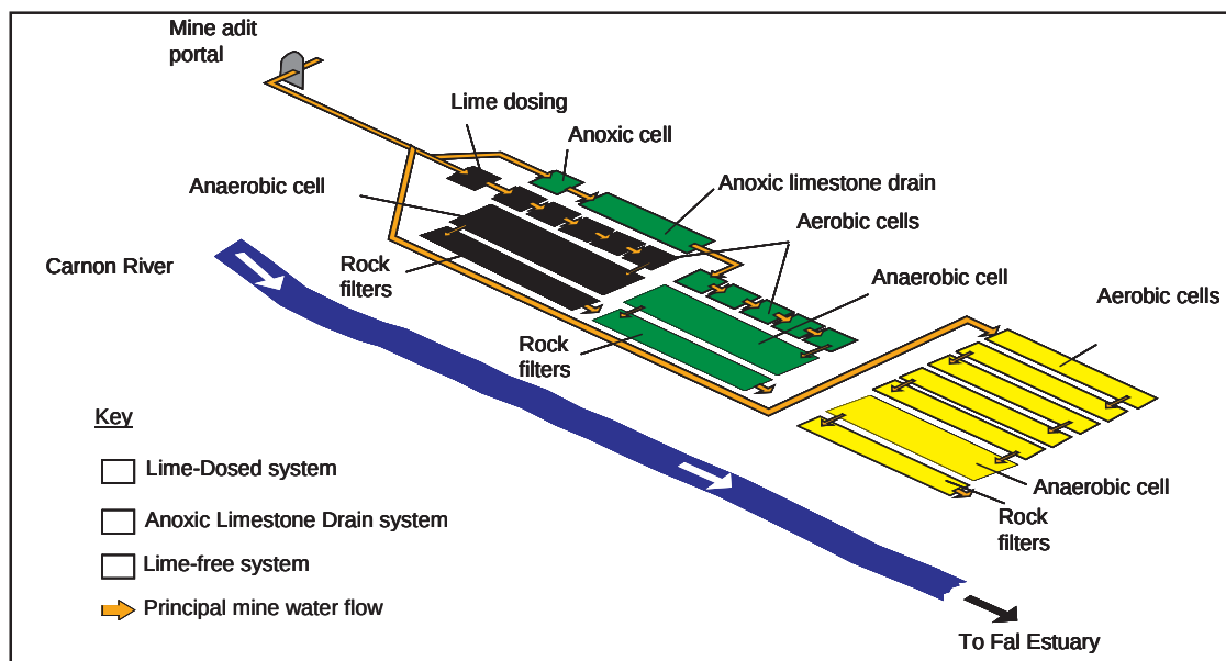
Figure 3: Schematic representation of the three systems within the pilot passive treatment system.
